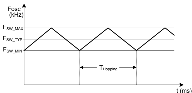
FIG.5 Frequency Hopping
