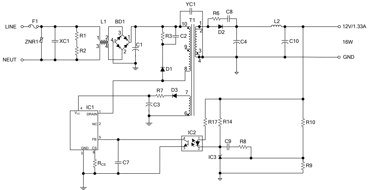
Fig.8 UTC UCS1657S Typical Application Circuit
