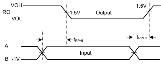
Fig. 9 Receiver Propagation Delays
