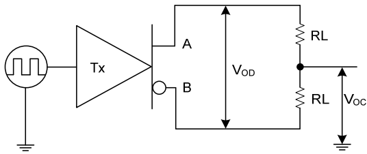
Fig. 1 Transmitter DC Test Circuit
