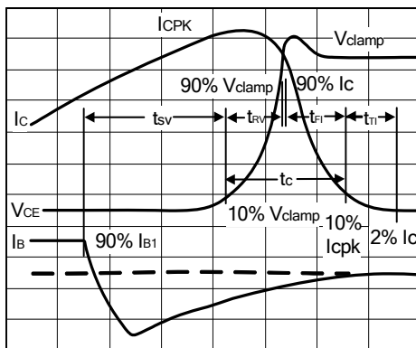
Figure 1. Inductive Switching Measurements
