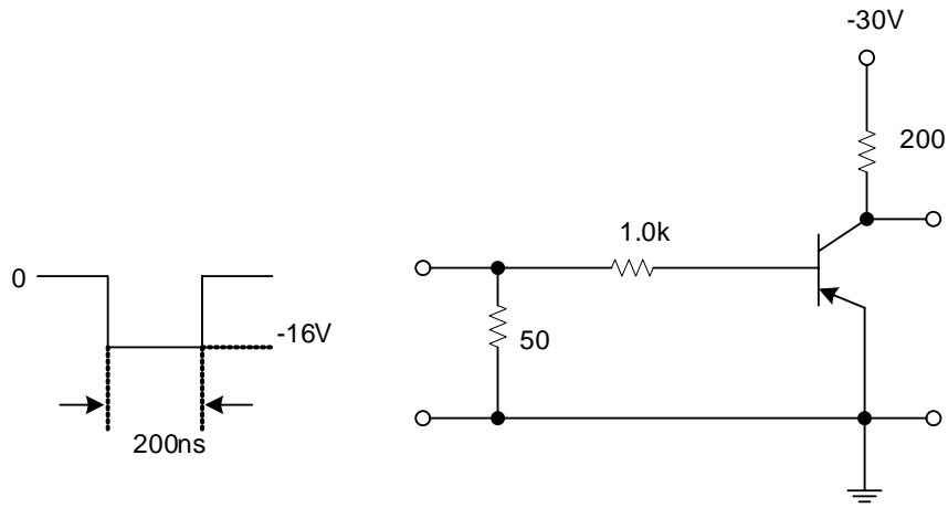
Fig. 1 Saturated Turn-On Switching Time Test Circuit
