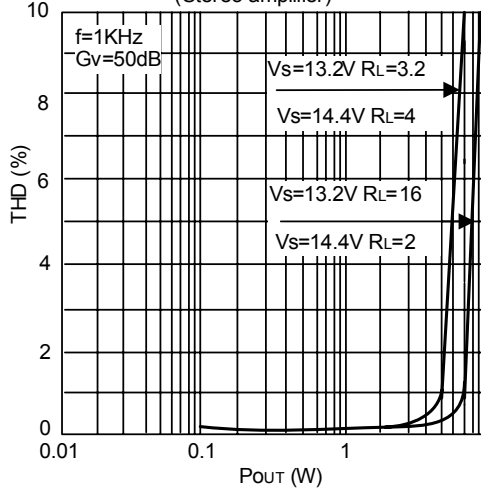
Figure 12. Distortion versus Output Power (Stereo amplifier)
