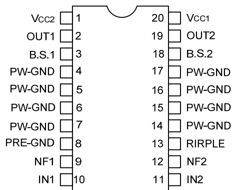
SOP-20
