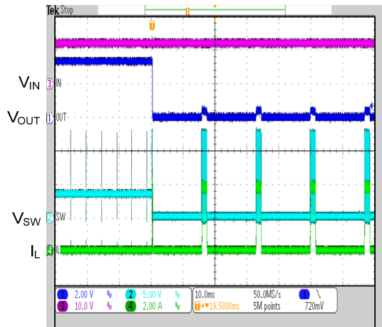
Short Circuit Entry and Recovery ( V_{IN}=12V , V_{OUT}=3.3V , I_{OUT}=0A )
