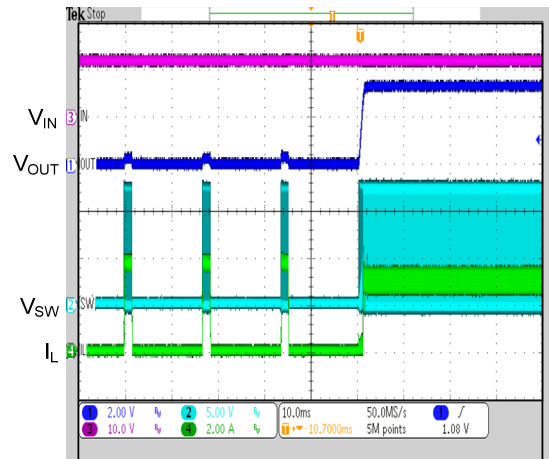
Short Circuit Entry and Recovery ( V_{IN}=12V , V_{OUT}=3.3V , I_{OUT}=3A )
