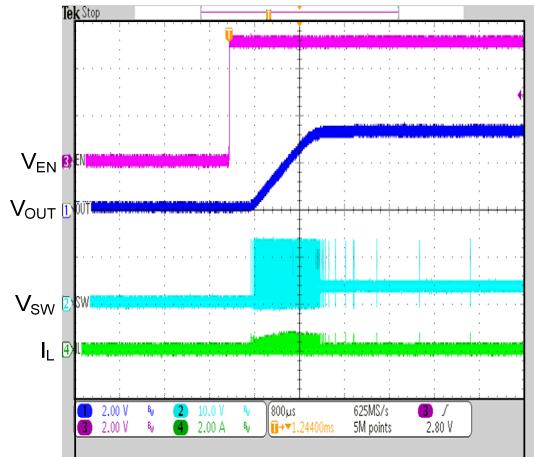
V_{EN} Power ON & Power OFF ( V_{IN}=12V , V_{OUT}=3.3V , V_{EN}=5V , I_{OUT}=0A )
