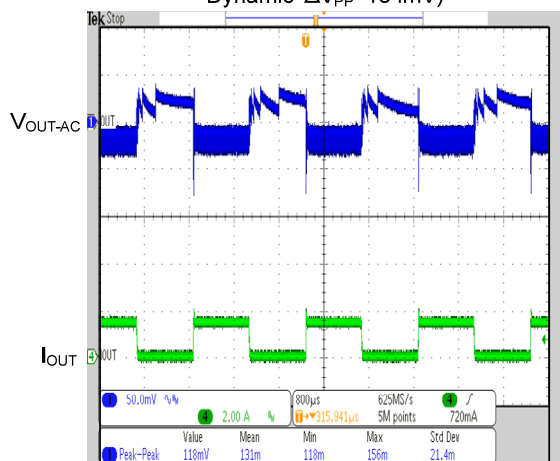
Dynamic Test ( V_{IN}=12V , V_{OUT}=3.3V , I_{OUT}=0\sim1.5A , Dynamic \Delta V_{PP}=134mV )
