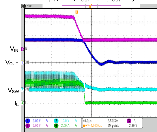
V_{IN} Power On & Power OFF ( V_{IN}=12V , V_{OUT}=3.3V , I_{OUT}=3A )
