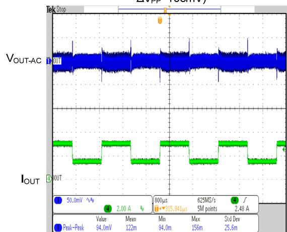
Dynamic Test ( V_{IN}=12V , V_{OUT}=3.3V , I_{OUT}=1.5\sim3A , Dynamic \Delta V_{PP}=108mV )
