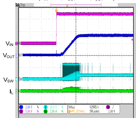
V_{IN} Power On & Power OFF ( V_{IN}=12V , V_{OUT}=3.3V , I_{OUT}=0A )
