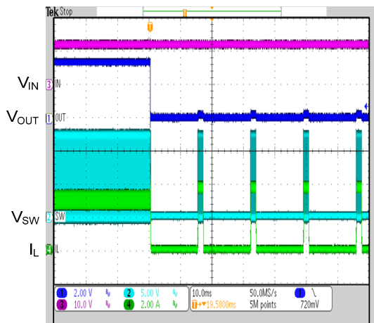
Short Circuit Entry and Recovery ( V_{IN}=12V , V_{OUT}=3V , I_{OUT}=0A )
