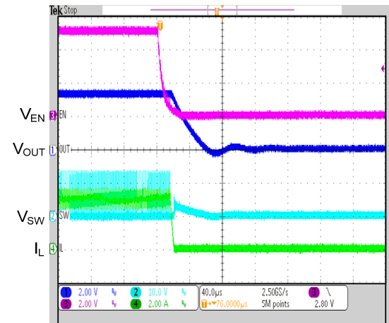
V_{EN} Power ON & Power OFF ( V_{IN}=12V , V_{OUT}=3.3V , V_{EN}=5V , I_{OUT}=0A )
