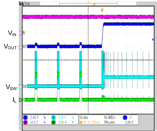
Short Circuit Entry and Recovery ( V_{IN}=12V , V_{OUT}=3.3V , I_{OUT}=0A )
