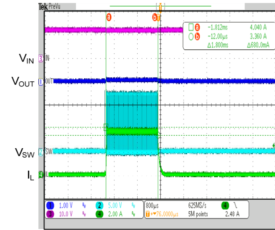
Short Circuit Entry and Recovery ( V_{IN}=12V , V_{OUT}=3.3V )
