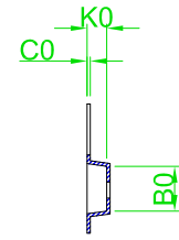
B-B' Section
